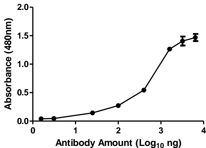
Figure 1. ELISA Dose Response curve using PtX™ Mouse Anti-CD20 (Biotin) Antibody from 64.0– 0.0156 ng/uL to detect 50 ng Human CD20-His-Avi Tag antigen. Experiments were performed in triplicate, with error bars representing standard deviation (SD).
