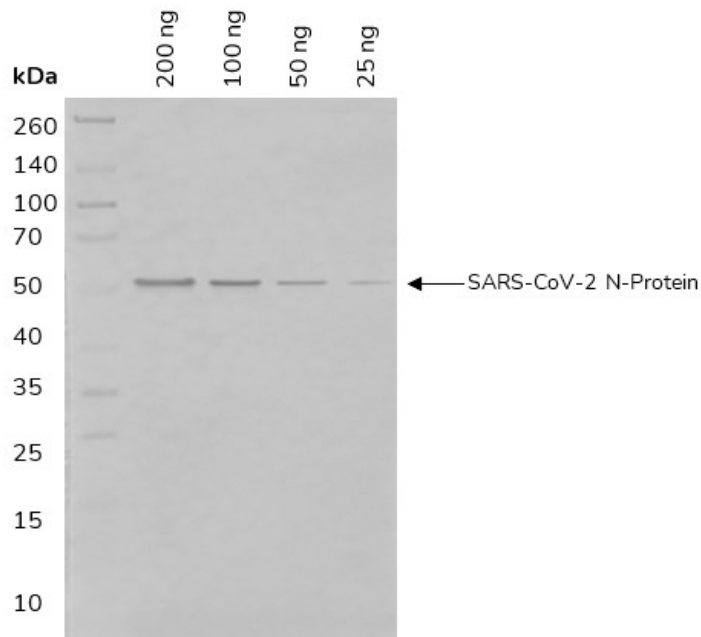
Figure 2. Western blot: decreasing amounts of SARS-CoV-2 N Protein (46 kDa) detected with PtX™ Human Anti-N (HuN5) (HRP) Antibody at 1: 1 000.
